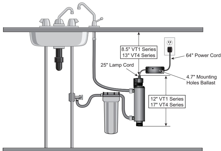
Figure 2 Disinfection System
